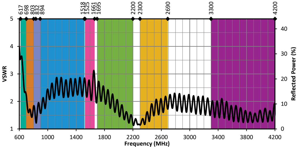
Figure 4. ANT-5GW-MMG1-SMA VSWR on Ground Plane
